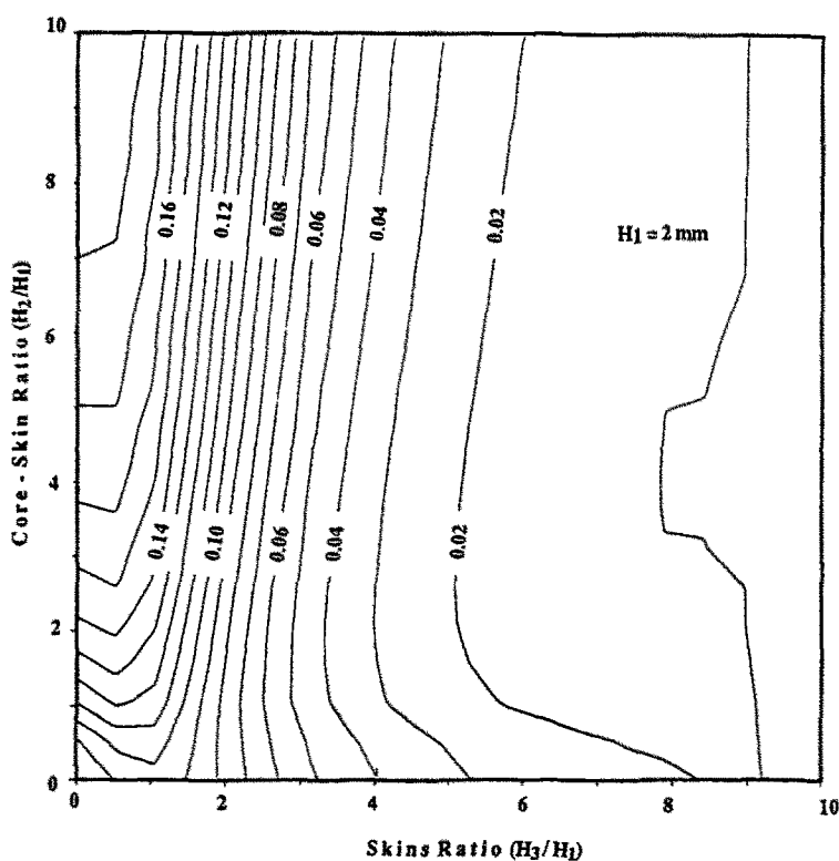
Fig. 10. Lines of equal damping of an unsymmetrical normalized sandwich beam ( H_1 = 2 mm).
